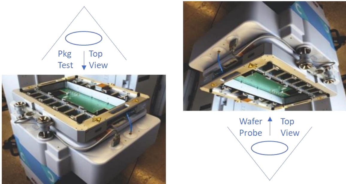
Figure 1: V93k CTH testhead with Multilane AT93000 system attached on top
