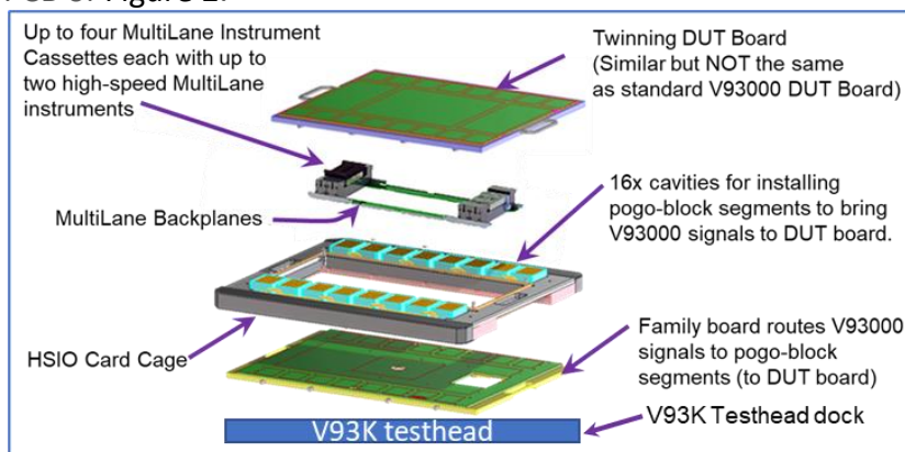
Figure 2: Building blocks of the Multilane AT93000 system
